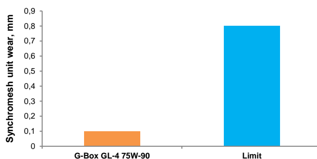
Synchronesh unit prolonged life*
